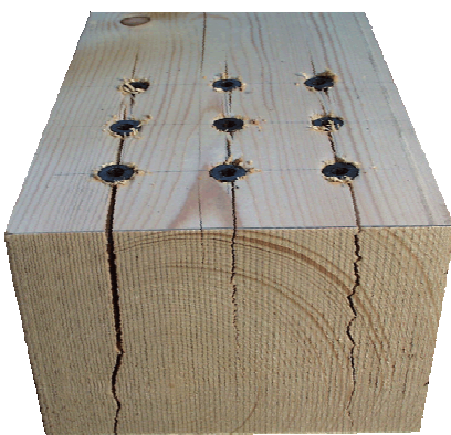
Figure 1: Splitting failure
