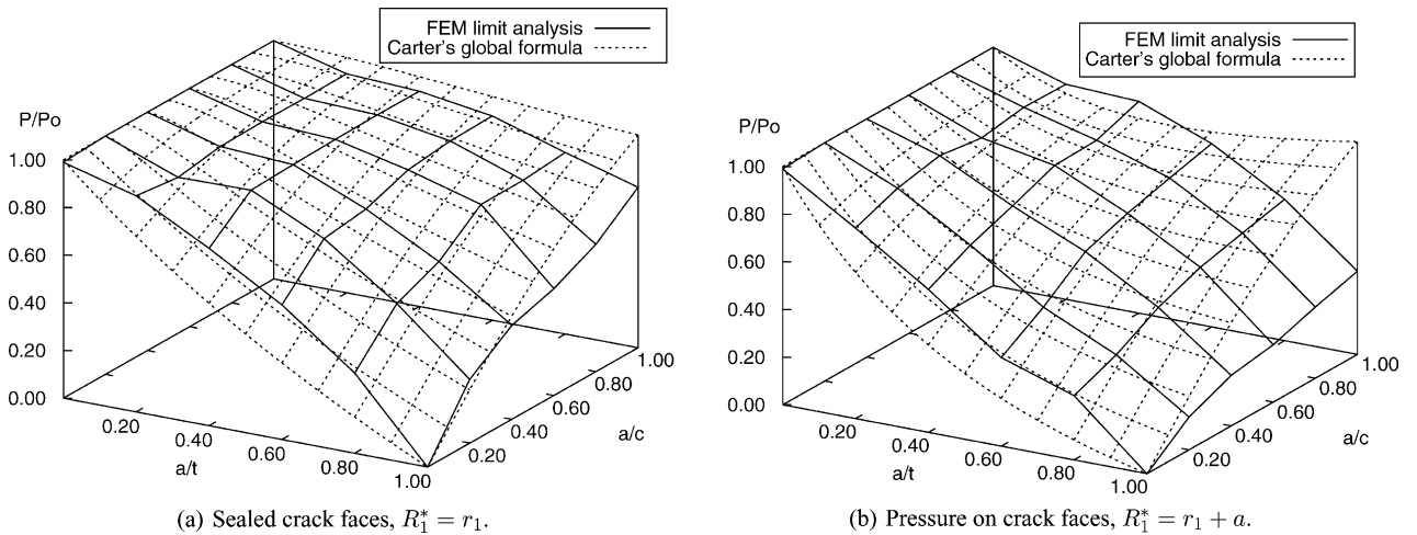
Fig. 3. Carter's global collapse pressure ( \bar{p}_{\text{global}} , Eq. (15)) compared with FEM limit analyses for internal defects in a thick pipe with r_2/r_1=2 . FEM —, formula ... . The pressures are normalised by p_0 .
