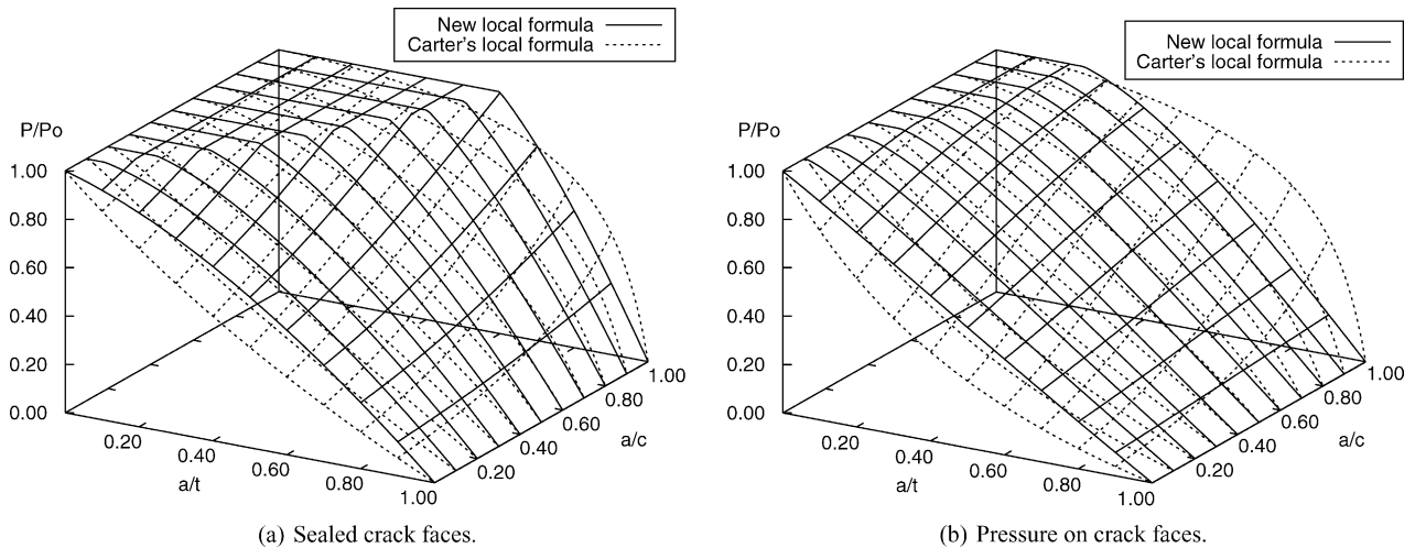
Fig. 9. New local collapse pressure ( p_{local} , Eqs. (24) and (25)) compared with Carter's local collapse pressure ( \bar{p}_{local} , Eqs. (22) and (23)) for internal defects in a thick pipe with r_2/r_1=2 . New formula —, Carter's formula ···. The pressures are normalised by p_0 .
